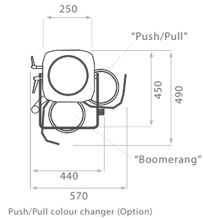
Push/Pull colour changer (Option)
